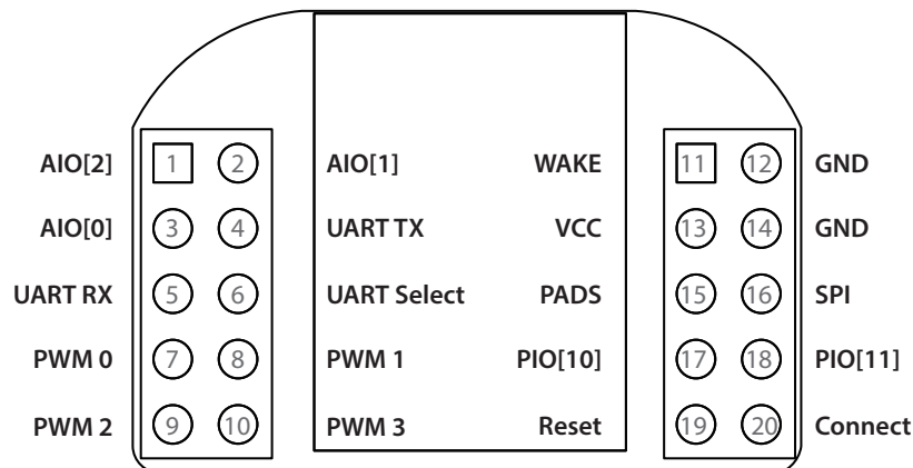
Pin configuration (Top View)
