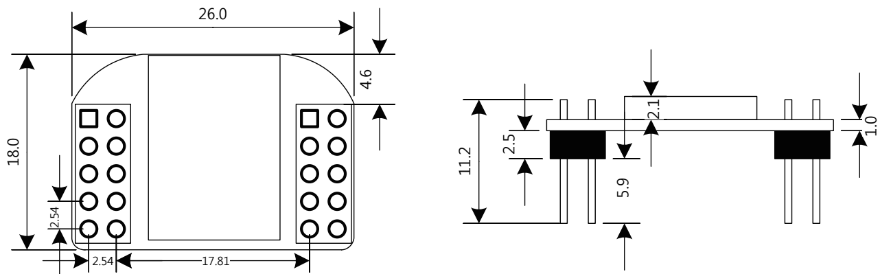
Outline Size
