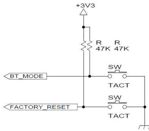
[Switch Interface]
