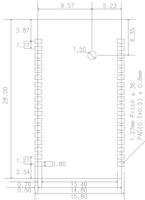
[BCD210SU, SC]
