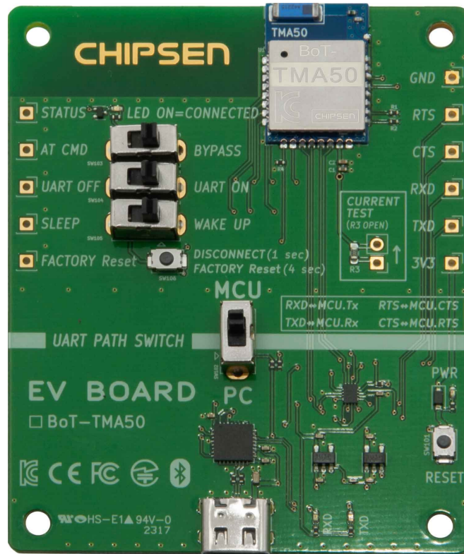
< EVB-TMA50 Product Image >
