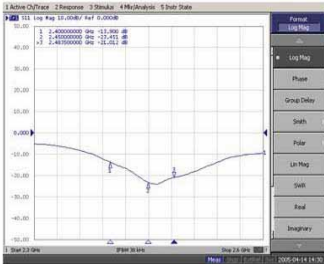
▲ Return Loss
